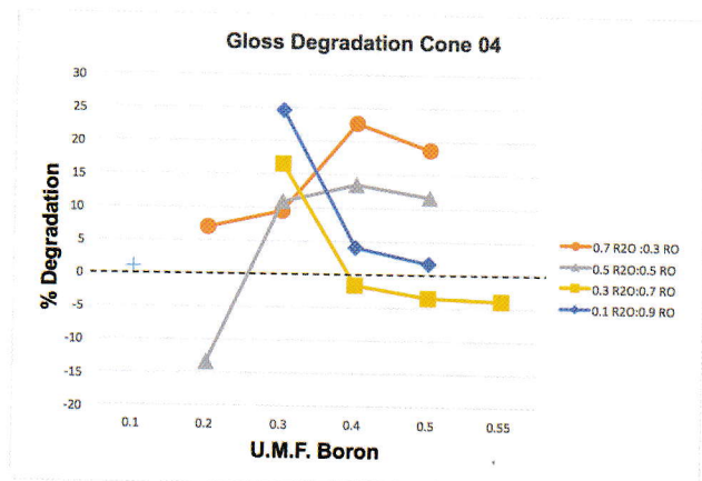
Figure 2. Documenting the washed degradation of several glazes based on boron and flux variation.
